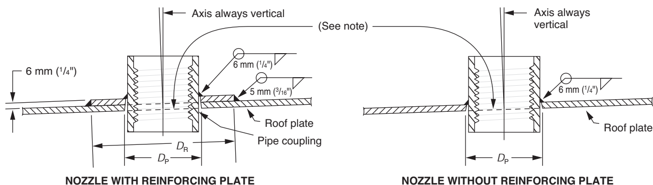
Figure 5-19—Flanged Roof Nozzles (See Table 5-14)
